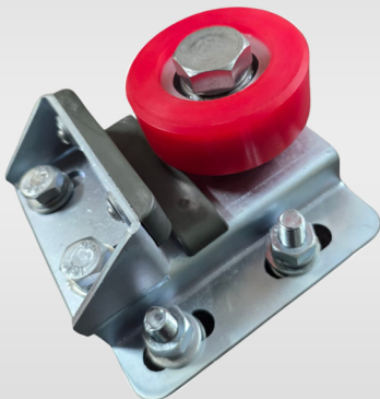
HYDRAULIC ROLLER GUIDE SHOE Ø 80 MM SKG-6
