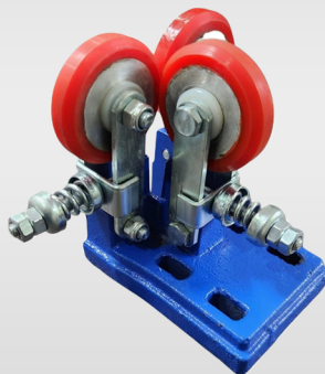
CASTED ROLLER GUIDE SHOE- SKG-8
