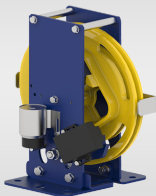
SPEED GOVERNER-TOP-MRL Ø 300 MM
