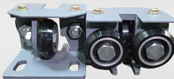
ROLLER GUIDE SHOE- Ø 50 MM-SKG 5
